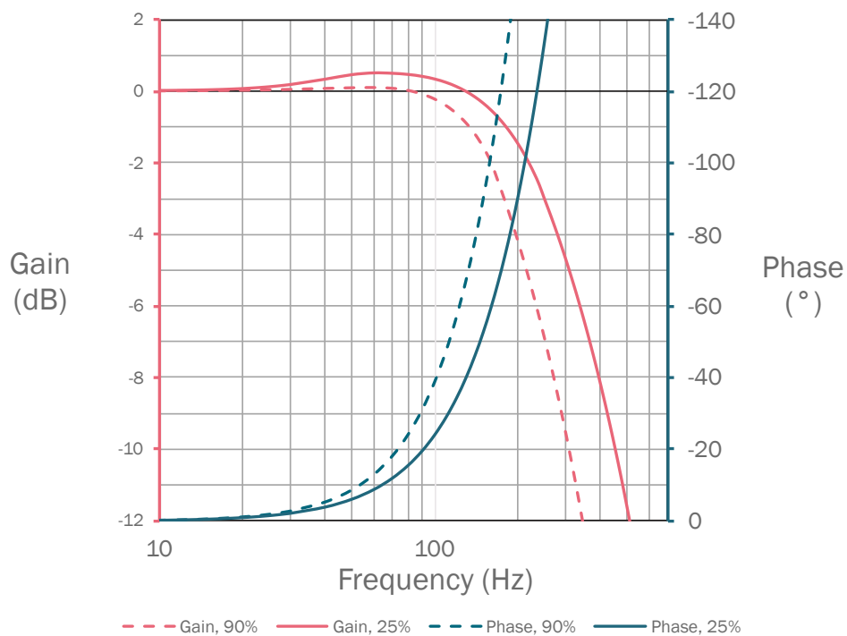
Frequency Response (1)
