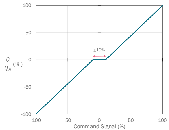
D - Deadband
